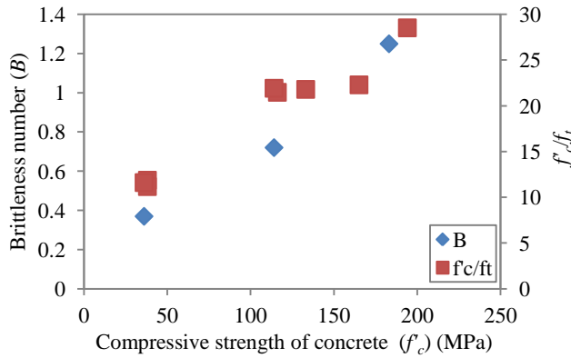
Figure 3: Brittleness of concrete
