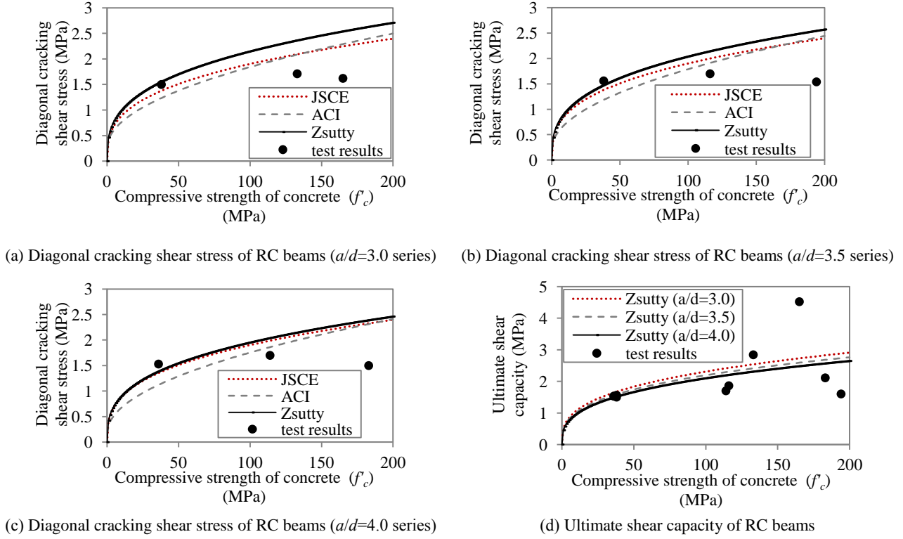
Figure 6: Shear stress of RC beams
