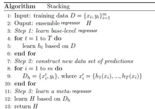
Fig. 2. Stacking regressor pseudocode [22]
