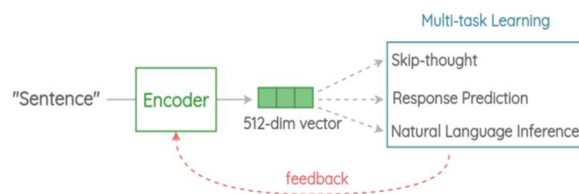
Fig. 1. USE embedding creation process [21]
