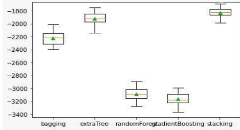
Fig. 5. Stacking regressor & individual model mean score comparison
